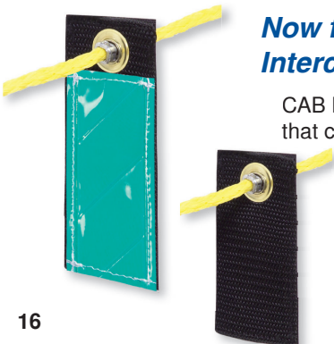
CAB Extra High Visibility Lifeline is easily seen from any direction in escapeways. Lifeline markers hang vertically so they can be seen for long distances up and down escapeways. Markers are flexible so miners' hands can slide easily over them.
