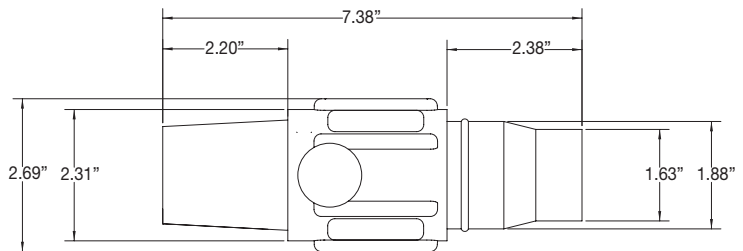
Female Connector
