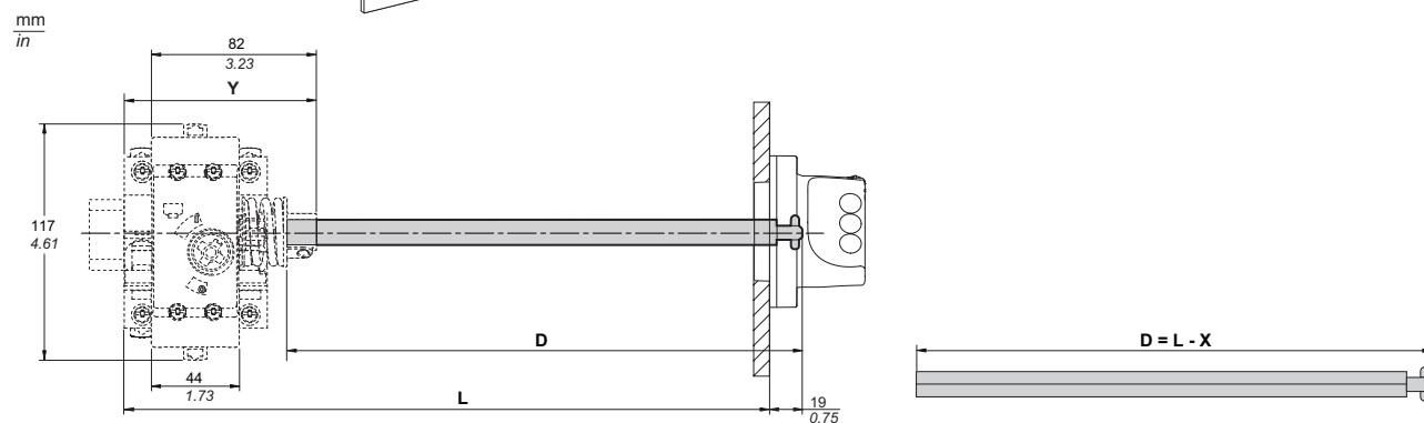
Rotary handle: side mounted control
