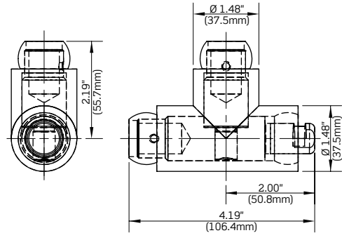
Tapping Tee Adapter
