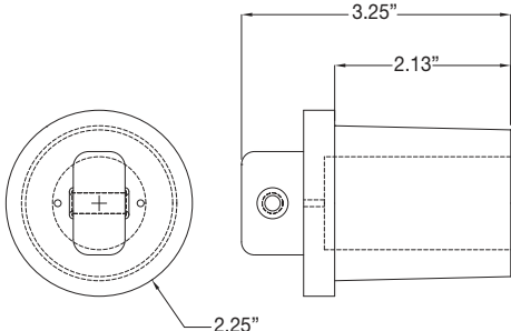
Male Cap
