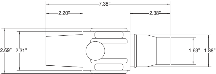
Female Connector
