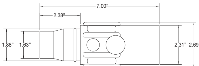
Male Connector
