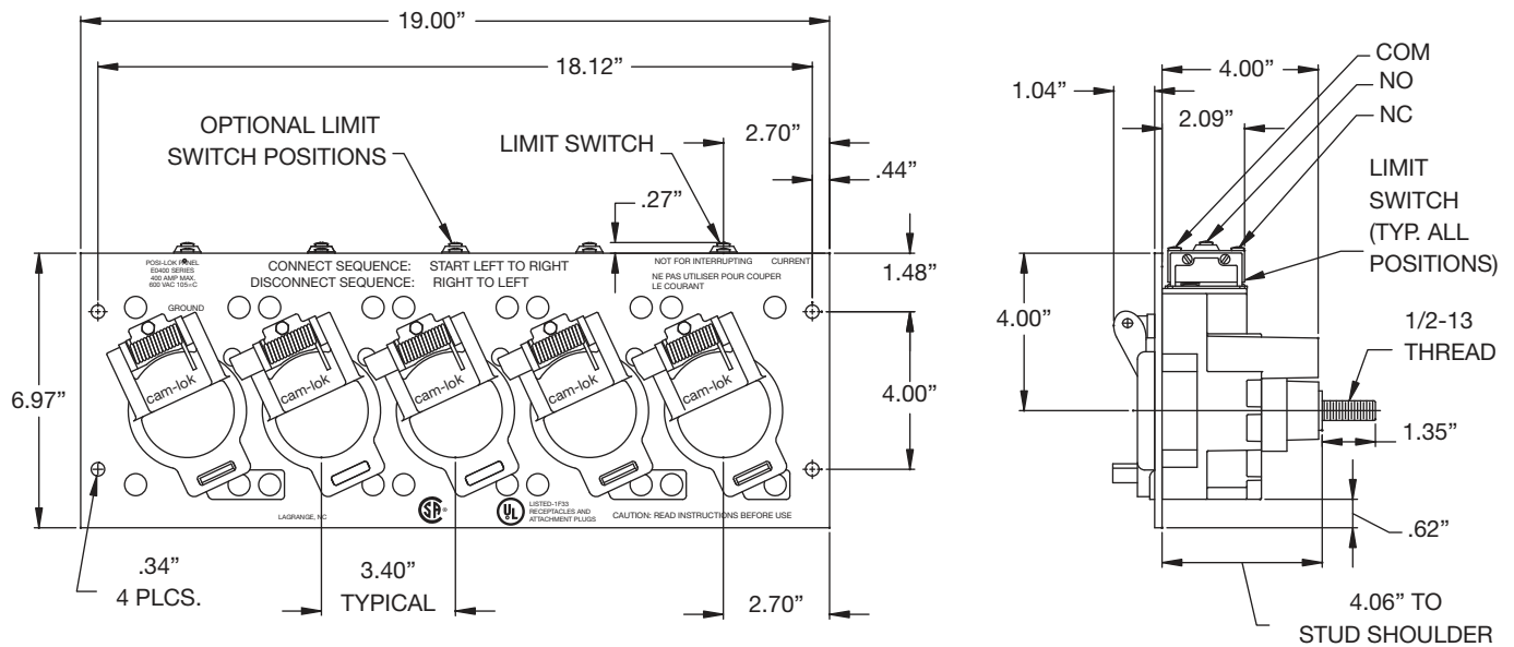
Panel with limit switch mounting dimensions
