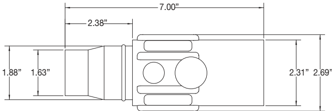
Male Connector
