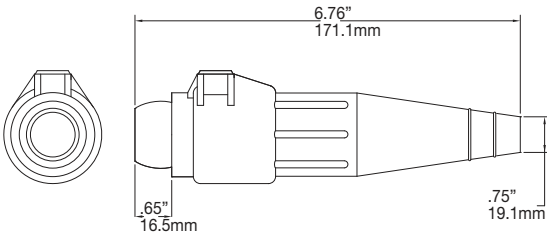
Female Connector
