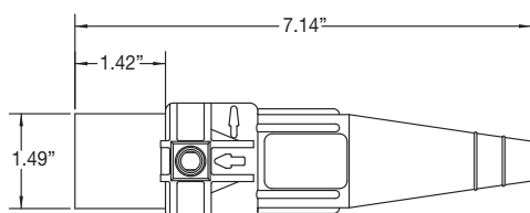
Male Connector
