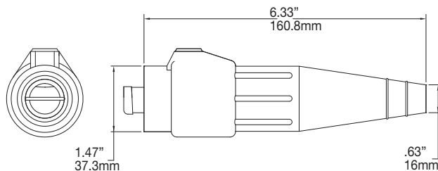
Male Connector
