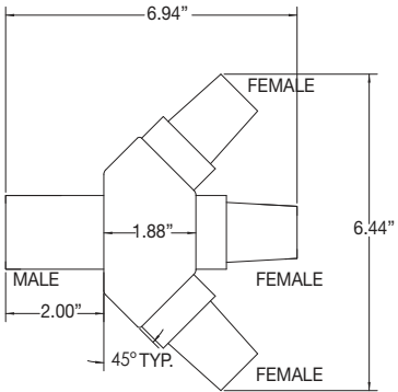
Three-fer Tapping Tee 45° M-F-F-F
