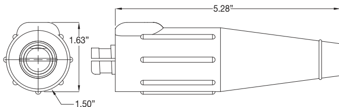
Male Plug
