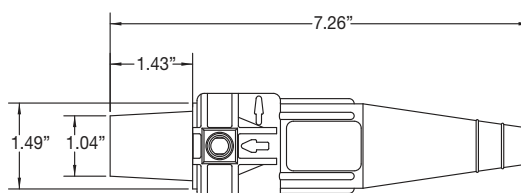
Female Connector
