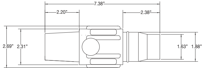
Female Connector
