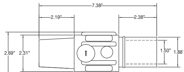
Female Connector
