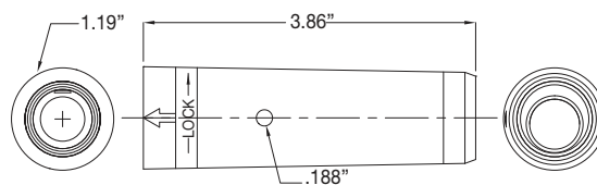
Male & Female High Temperature Plug
