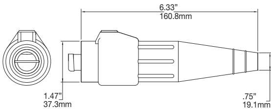
Male Connector
