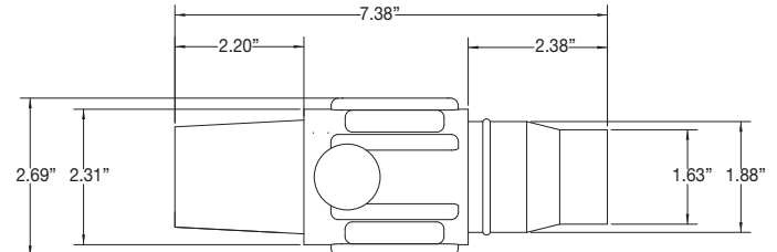
Female Connector
