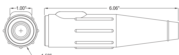
Female Plug
