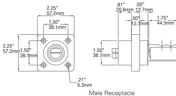
Male Receptacle
