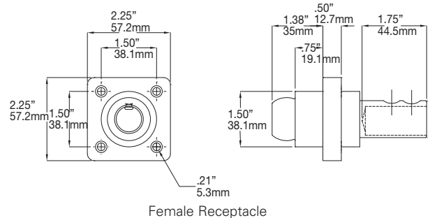
Female Receptacle
