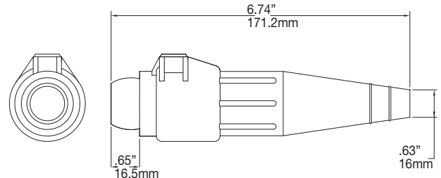
Female Connector
