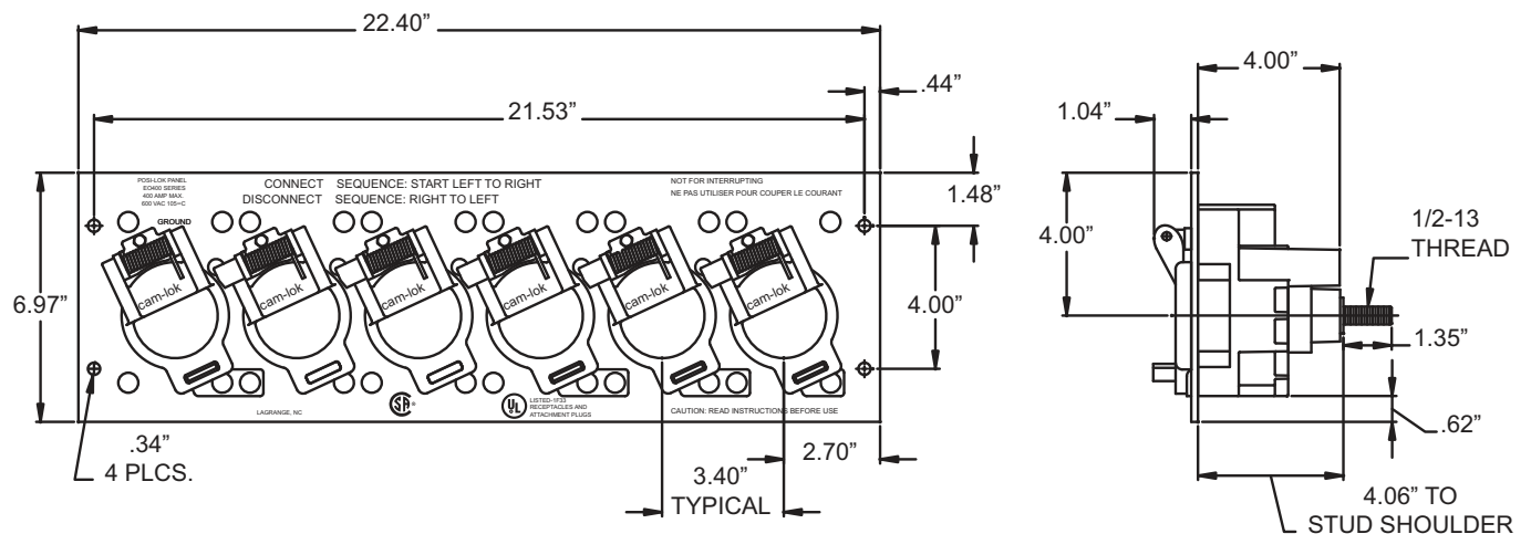
Panel without limit switch mounting dimensions
